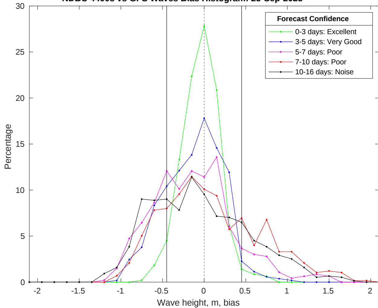
NDBC 44008 vs GFS Waves Bias Histogram: 25-Sep-2025
