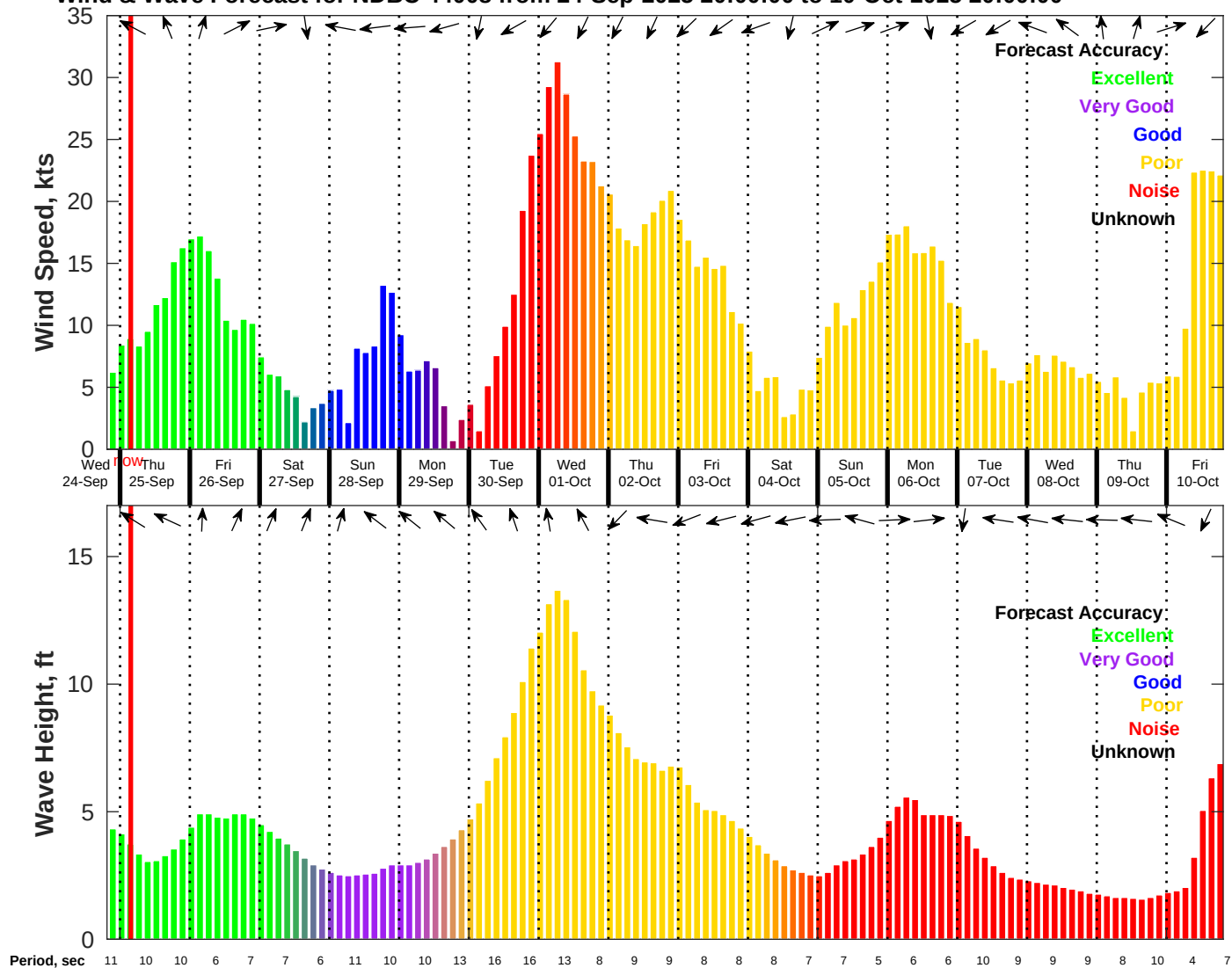
Wind & Wave Forecast for NDBC 44008 from 24-Sep-2025 20:00:00 to 10-Oct-2025 20:00:00
