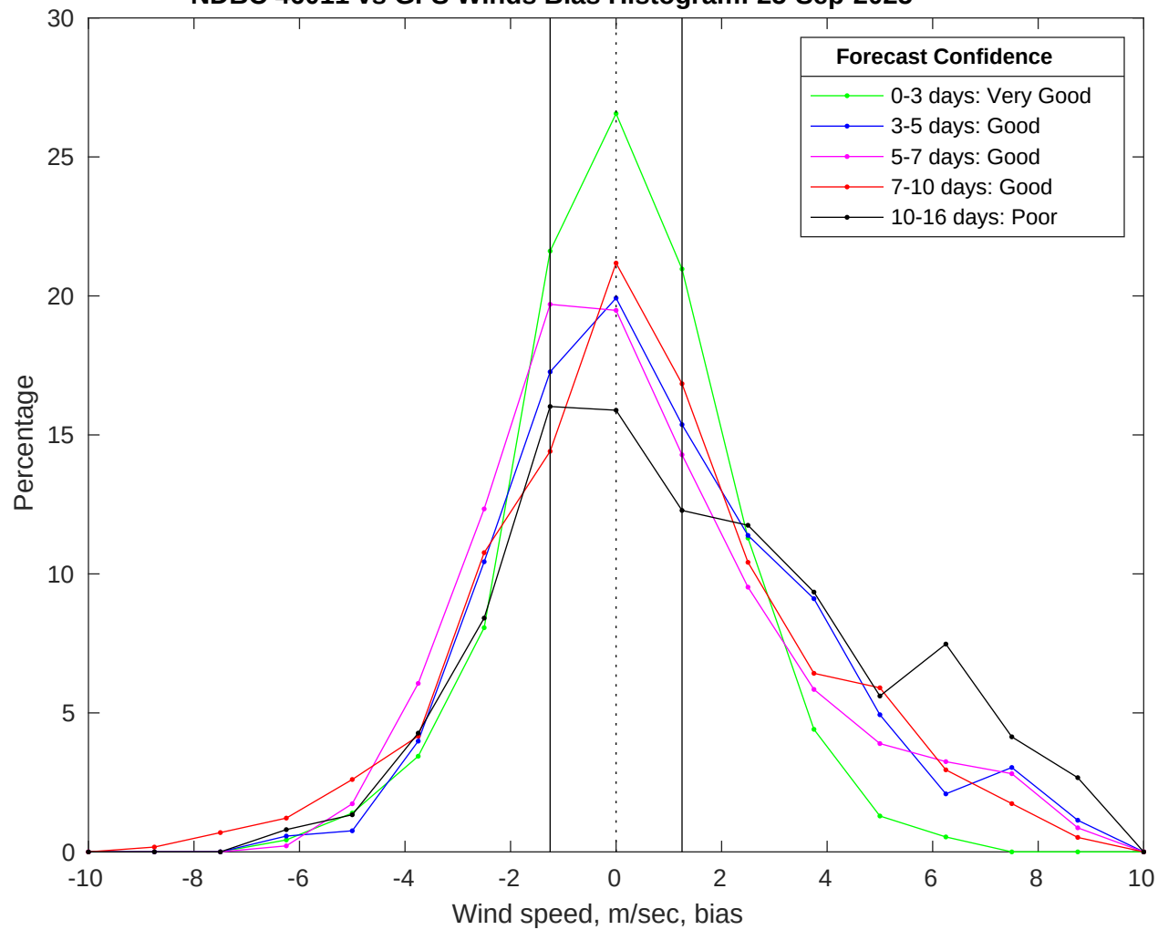
NDBC 46011 vs GFS Winds Bias Histogram: 25-Sep-2025
