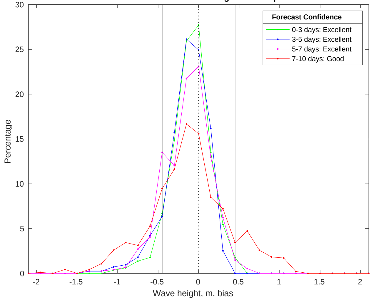
NDBC 46028 vs CMEMS Waves Bias Histogram: 25-Sep-2025
