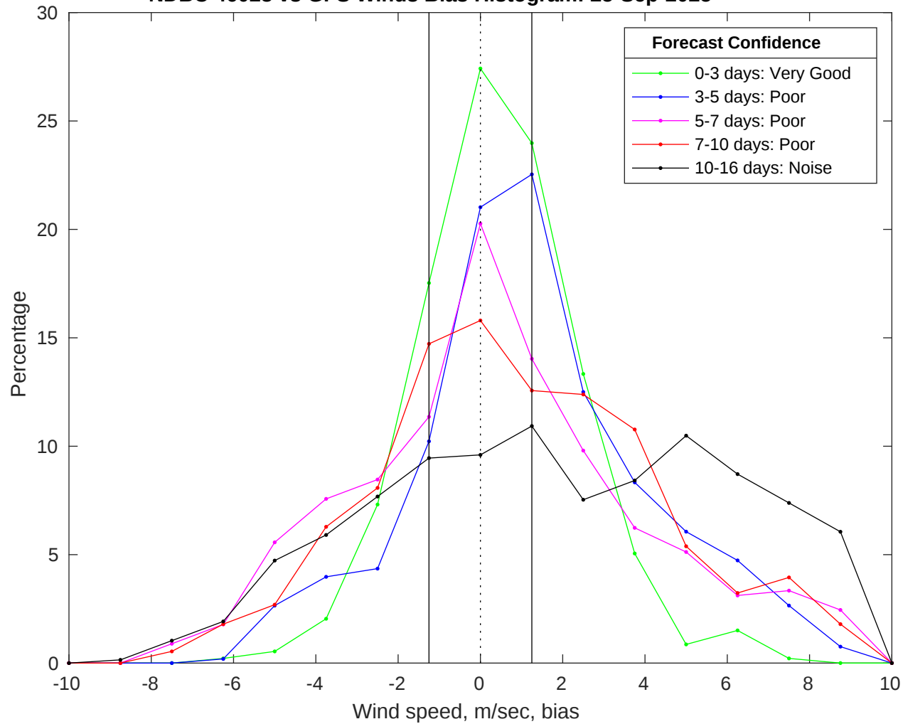
NDBC 46028 vs GFS Winds Bias Histogram: 25-Sep-2025
