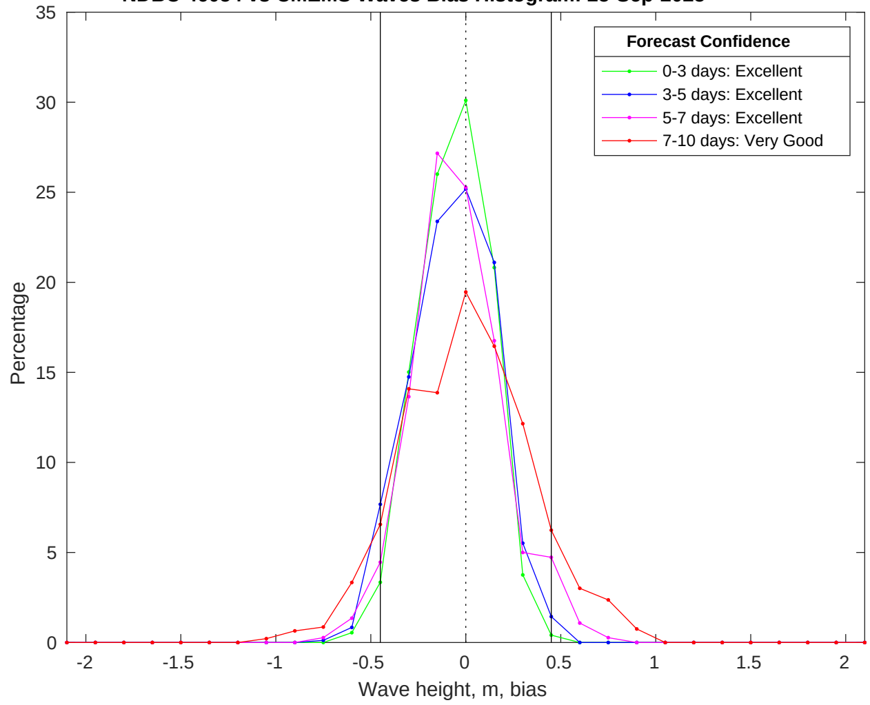
NDBC 46054 vs CMEMS Waves Bias Histogram: 25-Sep-2025
