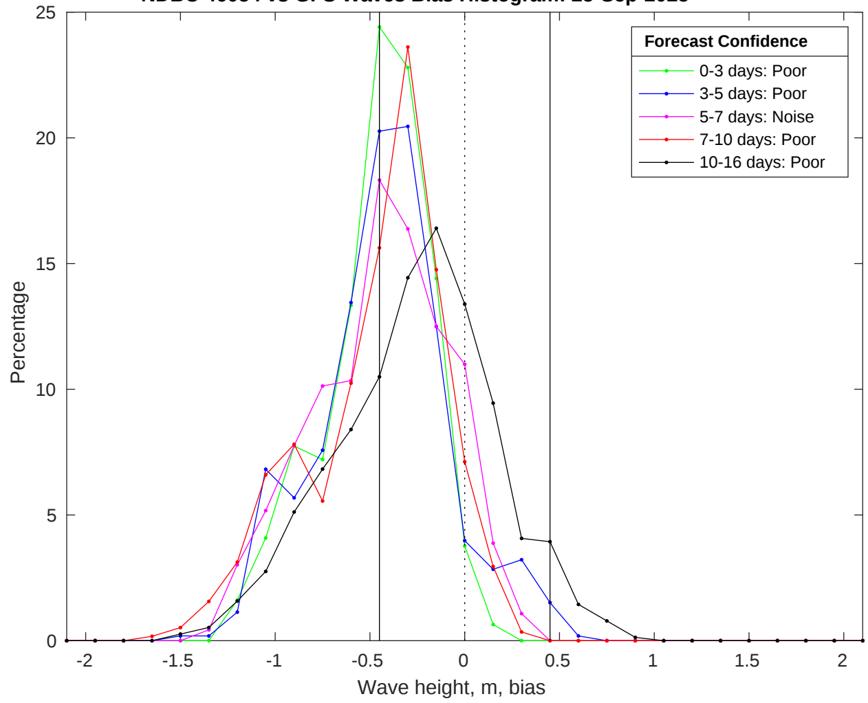
NDBC 46054 vs GFS Waves Bias Histogram: 25-Sep-2025
