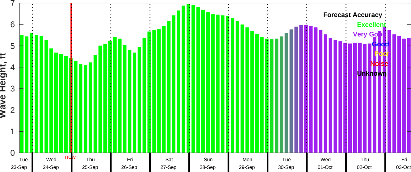
CMEMS Wave Forecast for NDBC 46054 from 23-Sep-2025 16:00:00 to 03-Oct-2025 16:00:00
