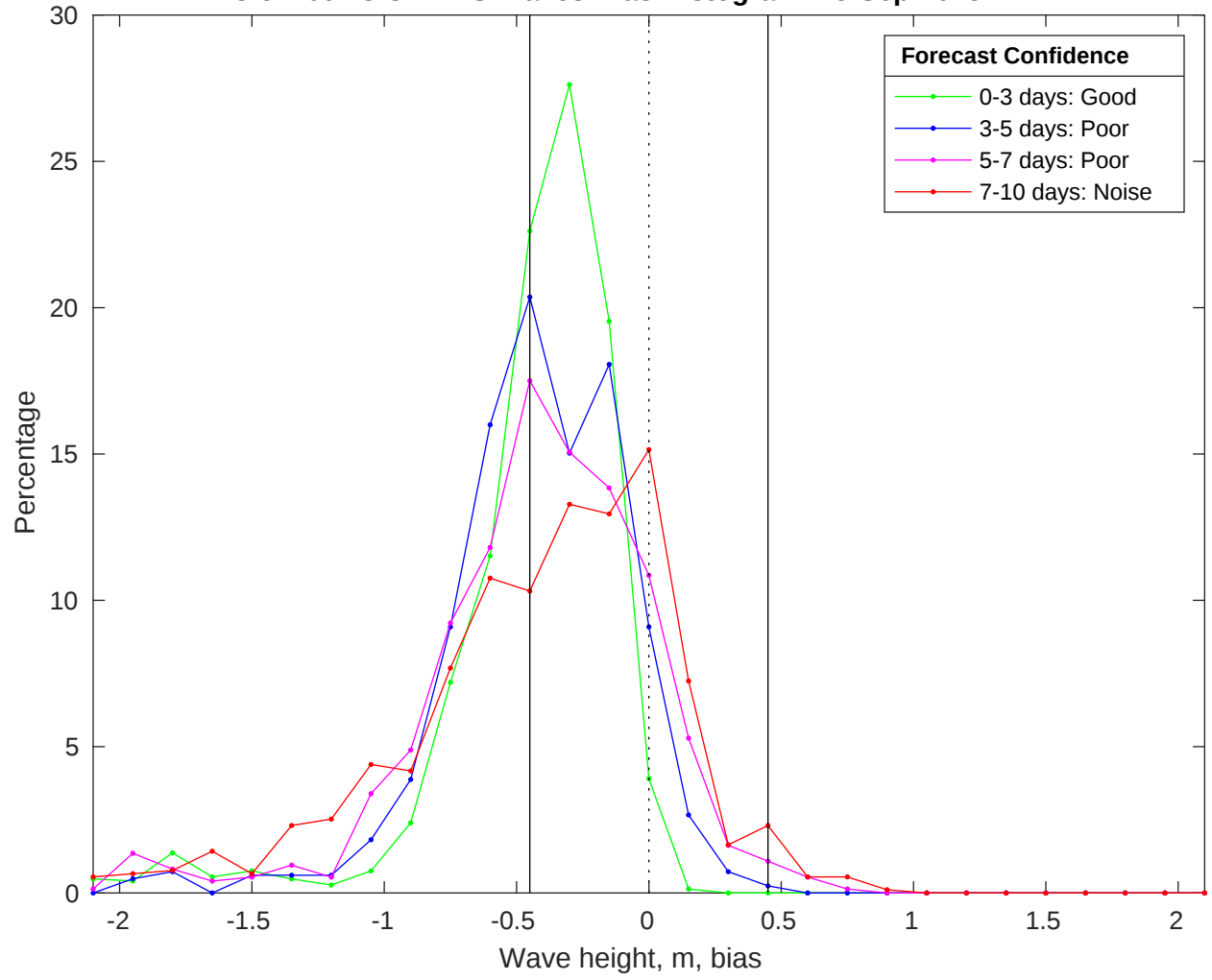
NDBC 51209 vs CMEMS Waves Bias Histogram: 25-Sep-2025
