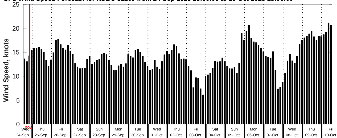
GFS Wind Speed Forecast for NDBC 51209 from 24-Sep-2025 13:00:00 to 10-Oct-2025 13:00:00
