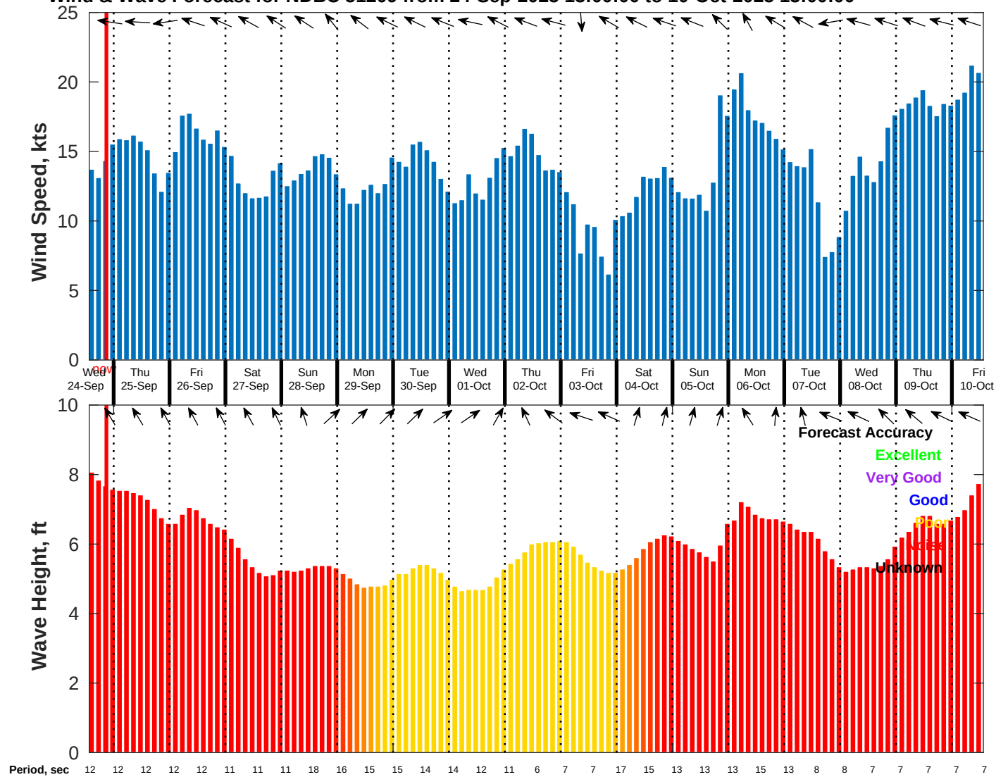
Wind & Wave Forecast for NDBC 51209 from 24-Sep-2025 13:00:00 to 10-Oct-2025 13:00:00
