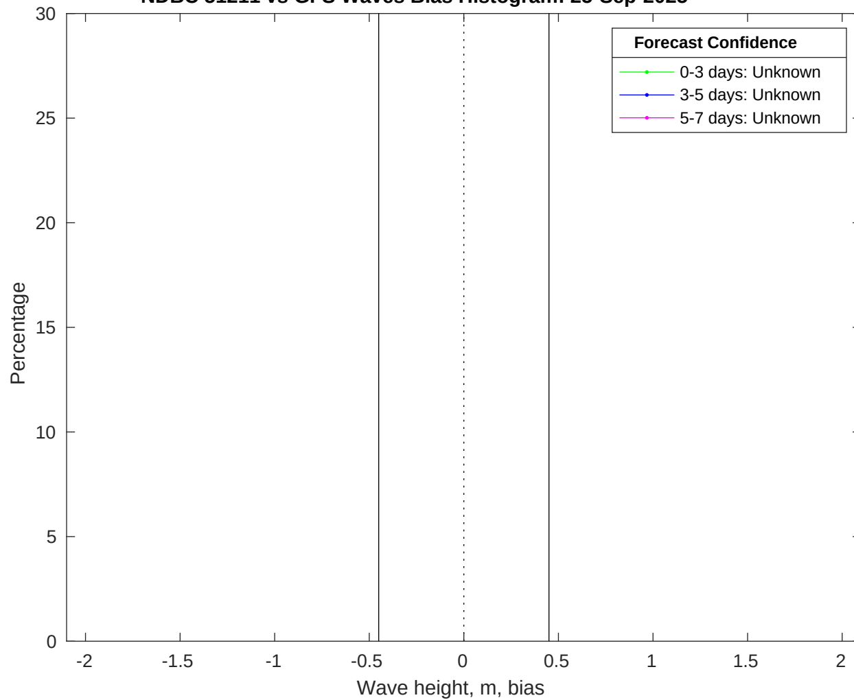
NDBC 51211 vs GFS Waves Bias Histogram: 25-Sep-2025
