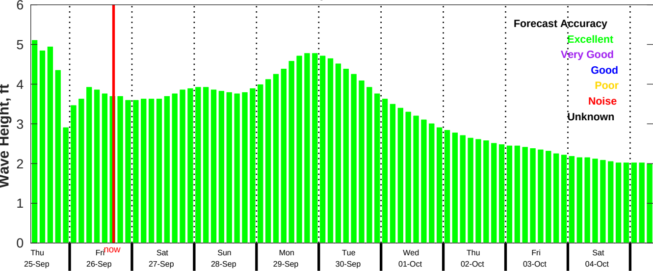
CMEMS Wave Forecast for NDBC 52212 from 24-Sep-2025 09:00:00 to 04-Oct-2025 09:00:00
