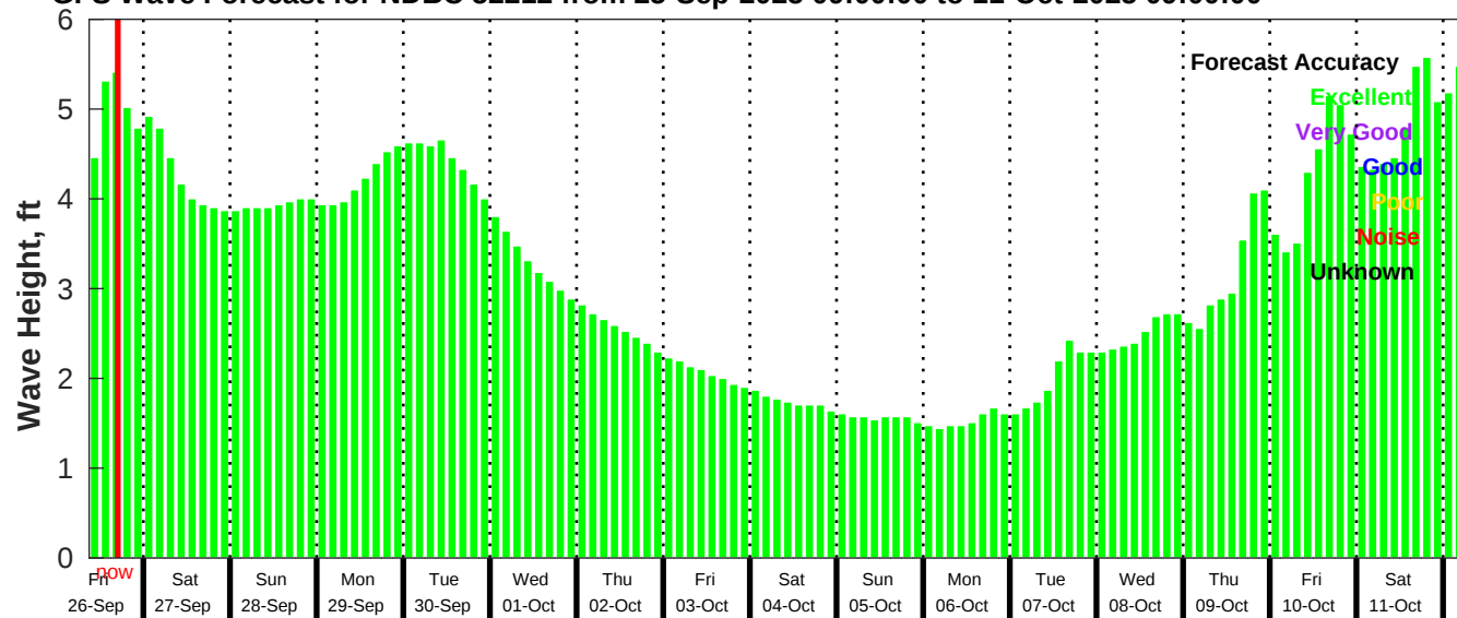
GFS Wave Forecast for NDBC 52212 from 25-Sep-2025 09:00:00 to 11-Oct-2025 09:00:00
