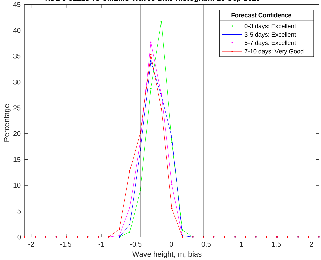
NDBC 52213 vs CMEMS Waves Bias Histogram: 25-Sep-2025
