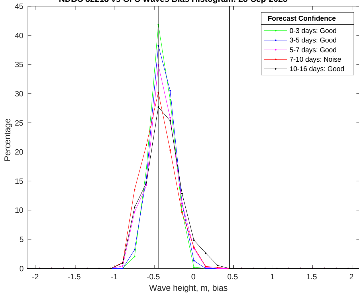
NDBC 52213 vs GFS Waves Bias Histogram: 25-Sep-2025
