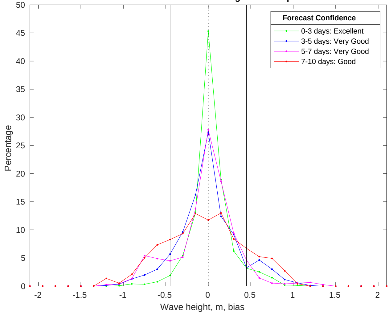
NDBC 41004 vs CMEMS Waves Bias Histogram: 26-Sep-2025
