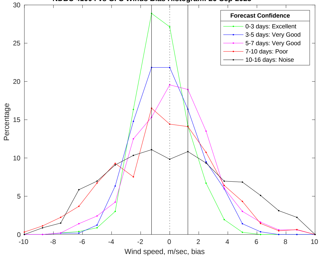
NDBC 41004 vs GFS Winds Bias Histogram: 26-Sep-2025
