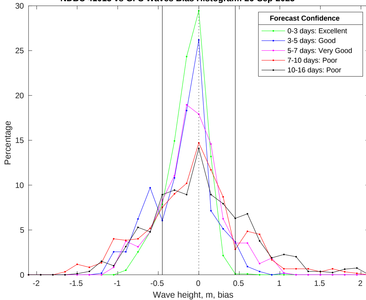
NDBC 41013 vs GFS Waves Bias Histogram: 26-Sep-2025
