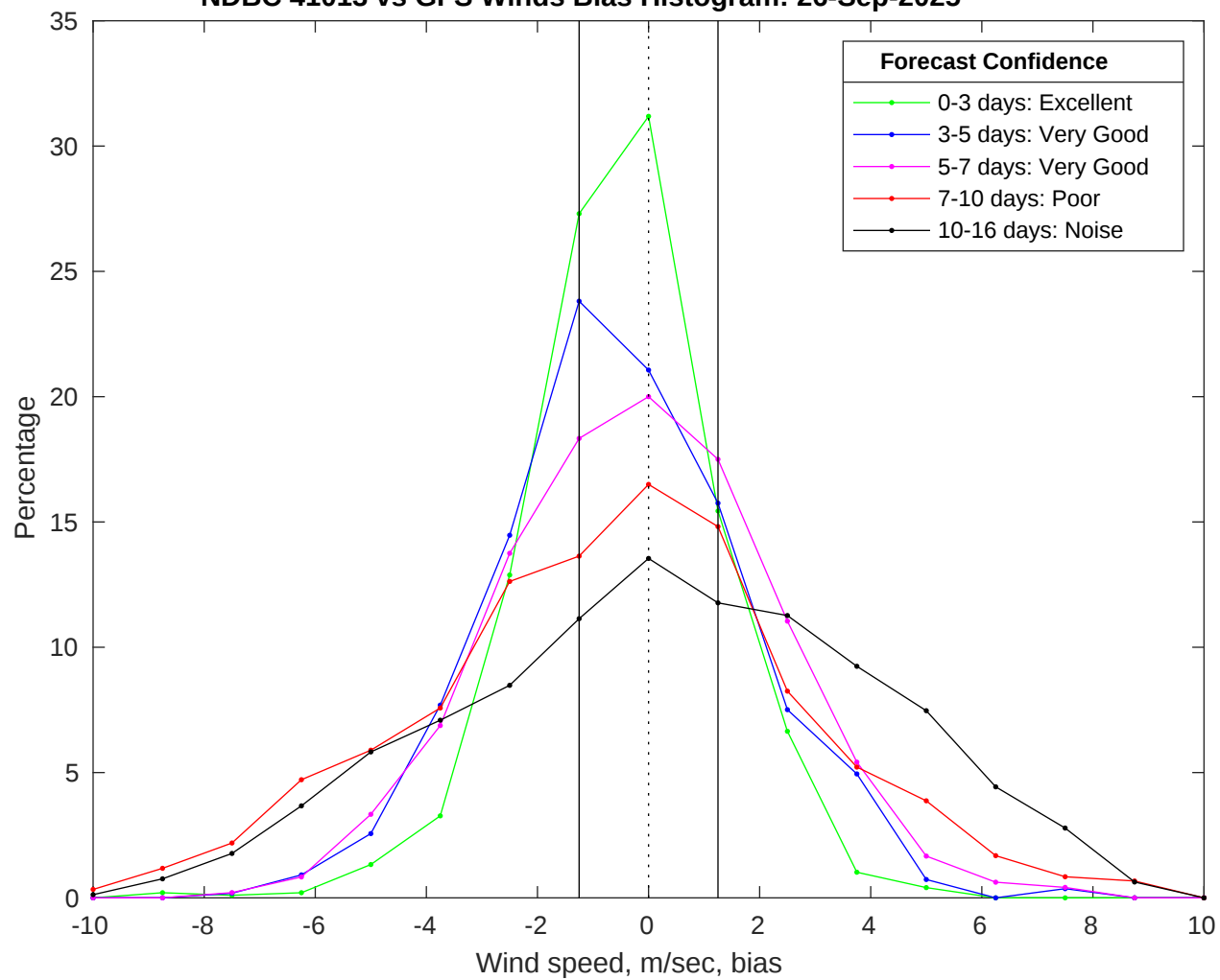
NDBC 41013 vs GFS Winds Bias Histogram: 26-Sep-2025
