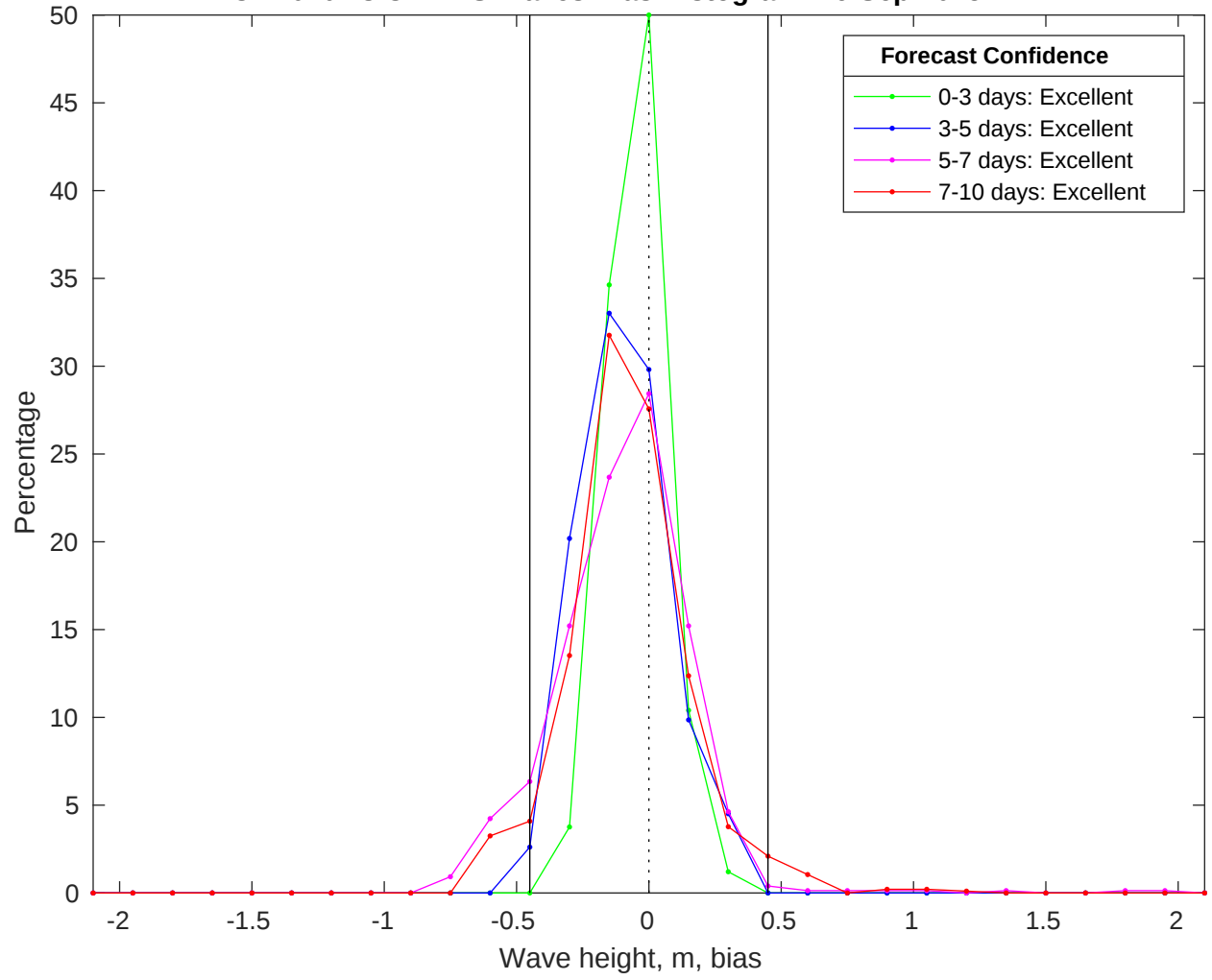
NDBC 41040 vs CMEMS Waves Bias Histogram: 26-Sep-2025
