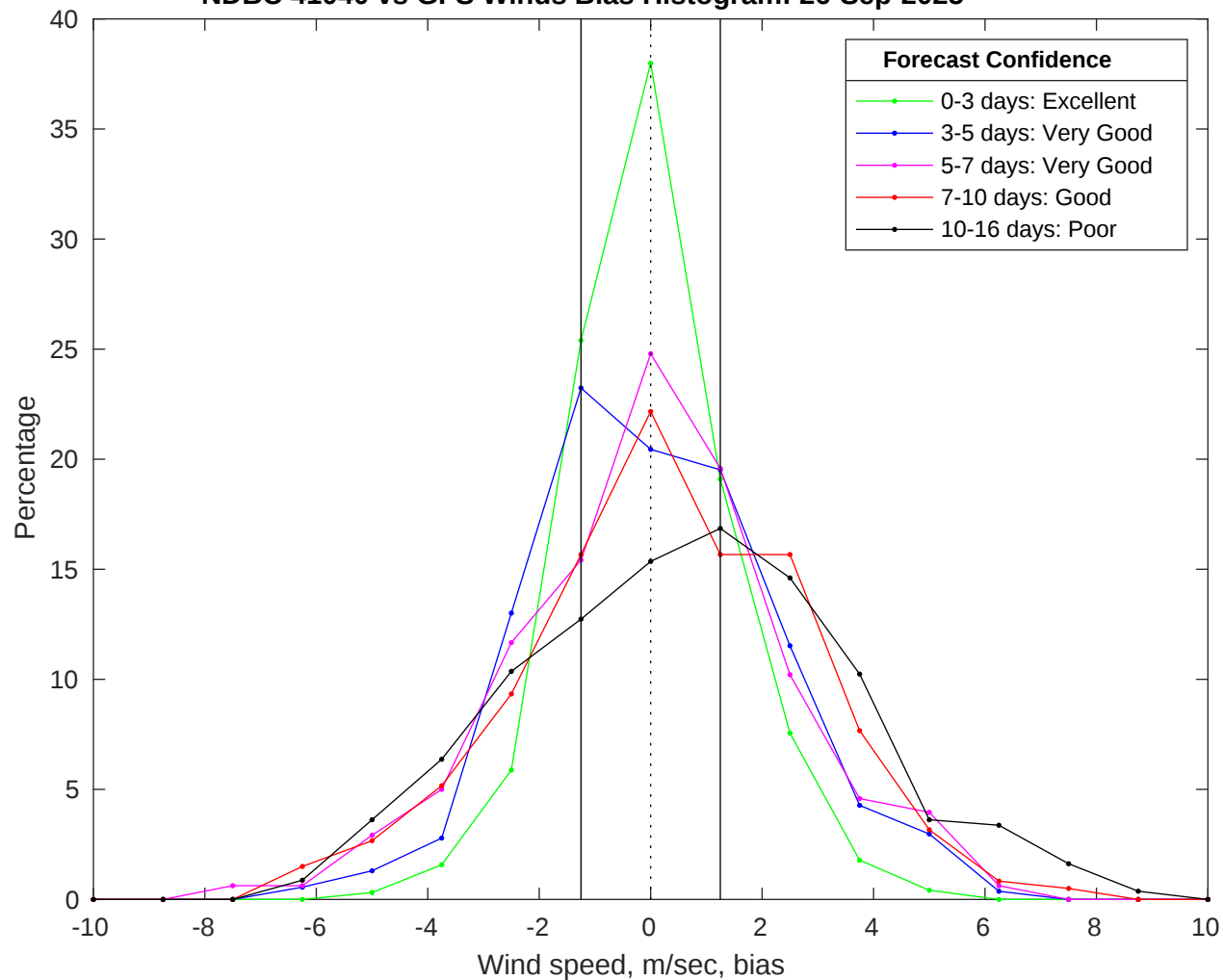
NDBC 41040 vs GFS Winds Bias Histogram: 26-Sep-2025
