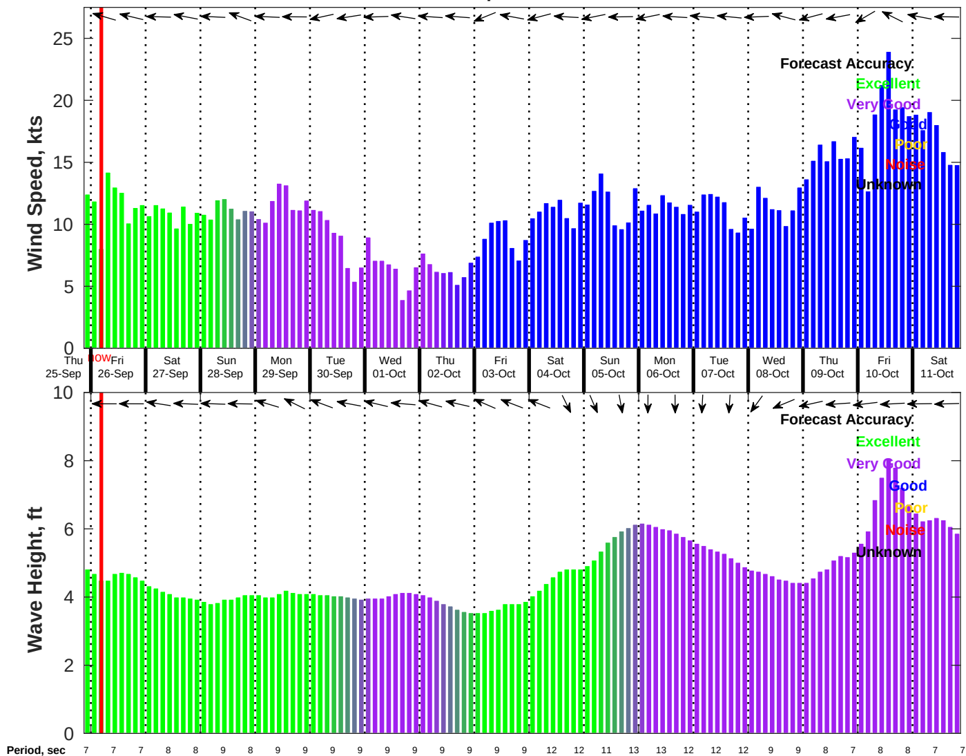
Wind & Wave Forecast for NDBC 41040 from 25-Sep-2025 21:00:00 to 11-Oct-2025 21:00:00
