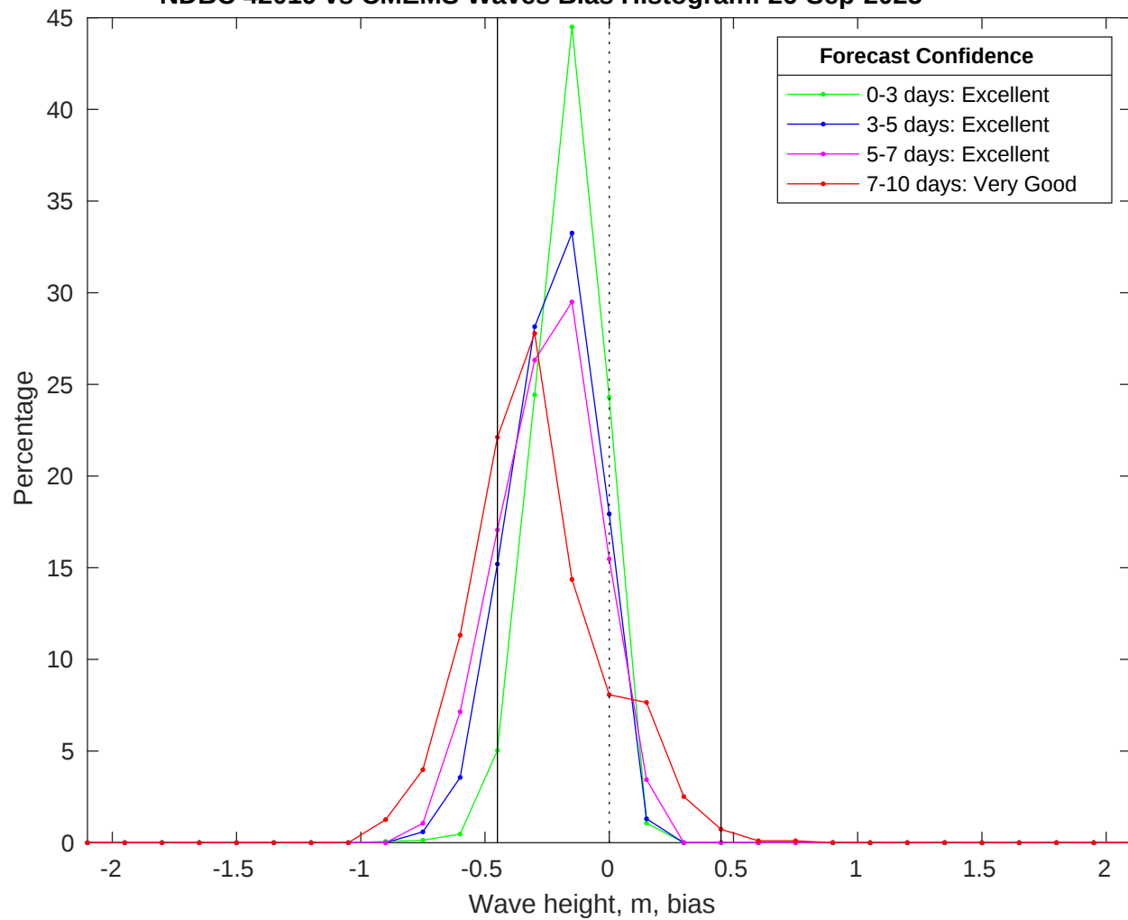
NDBC 42019 vs CMEMS Waves Bias Histogram: 26-Sep-2025
