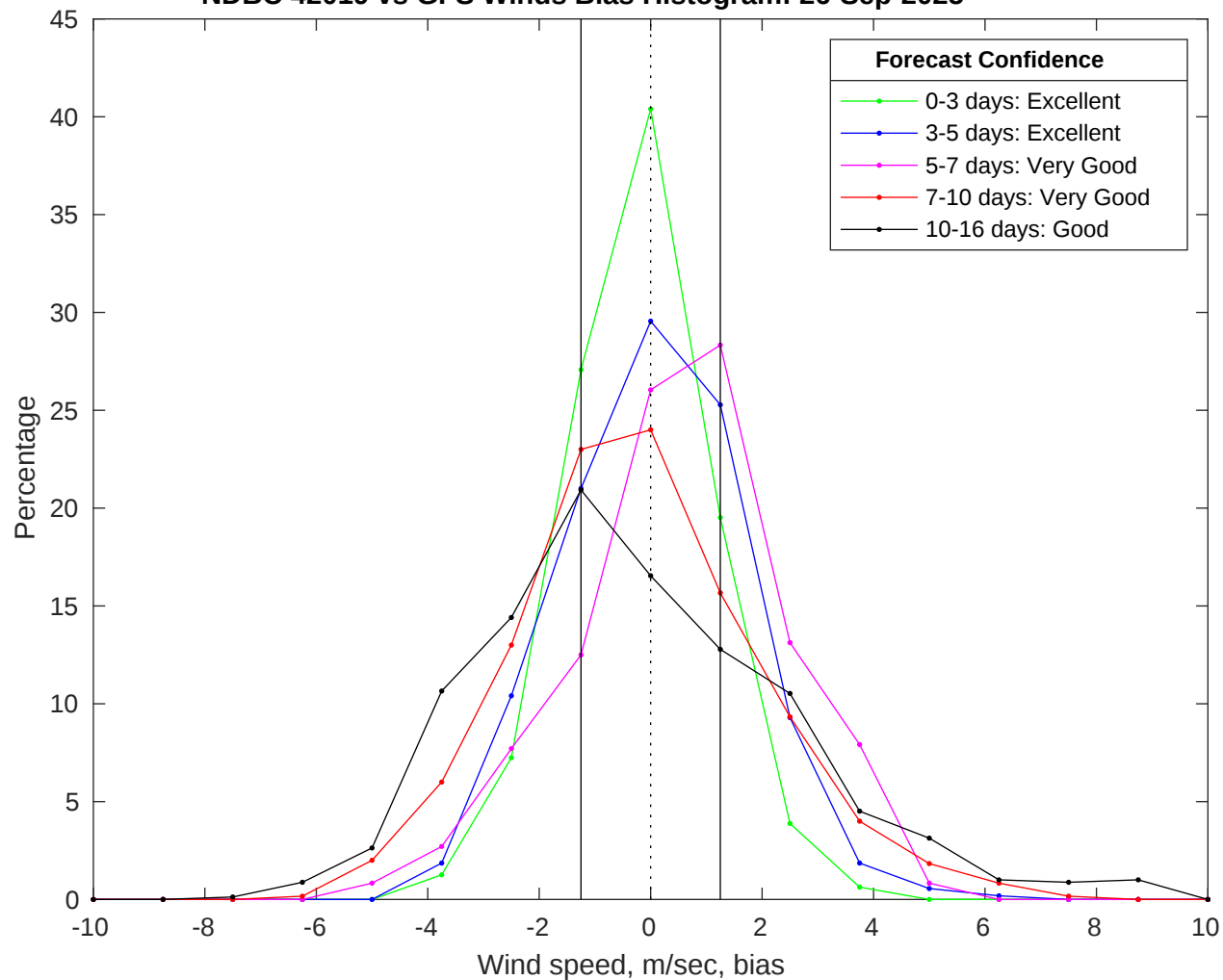
NDBC 42019 vs GFS Winds Bias Histogram: 26-Sep-2025
