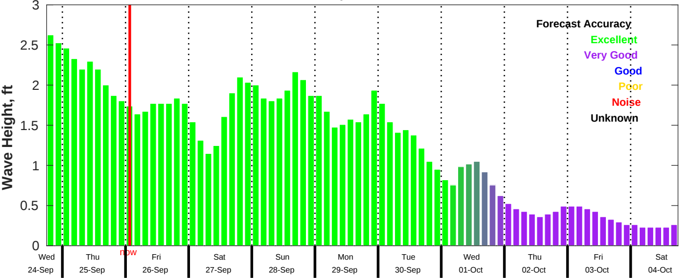
CMEMS Wave Forecast for NDBC 42019 from 24-Sep-2025 18:00:00 to 04-Oct-2025 18:00:00
