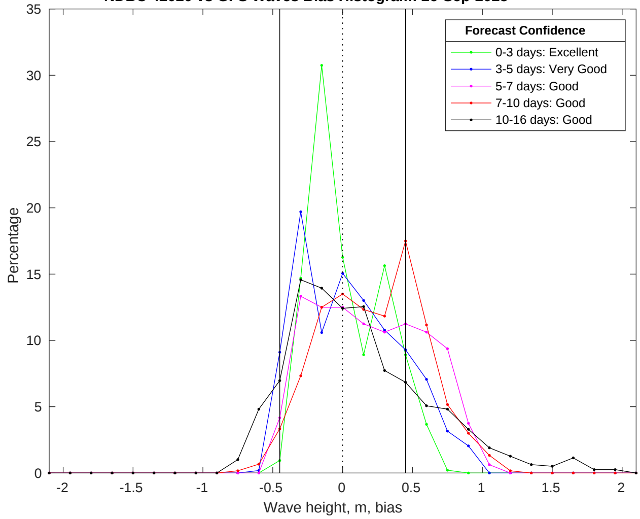
NDBC 42020 vs GFS Waves Bias Histogram: 26-Sep-2025
