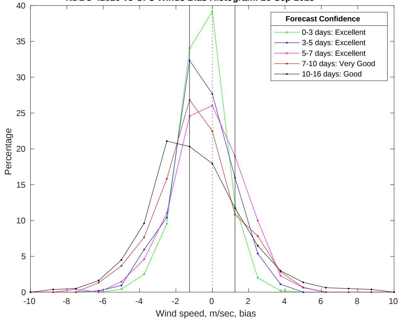
NDBC 42020 vs GFS Winds Bias Histogram: 26-Sep-2025
