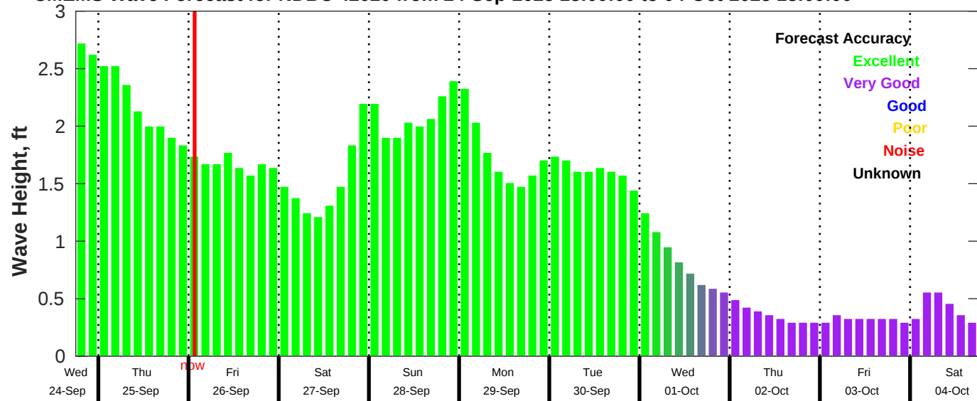
CMEMS Wave Forecast for NDBC 42020 from 24-Sep-2025 18:00:00 to 04-Oct-2025 18:00:00
