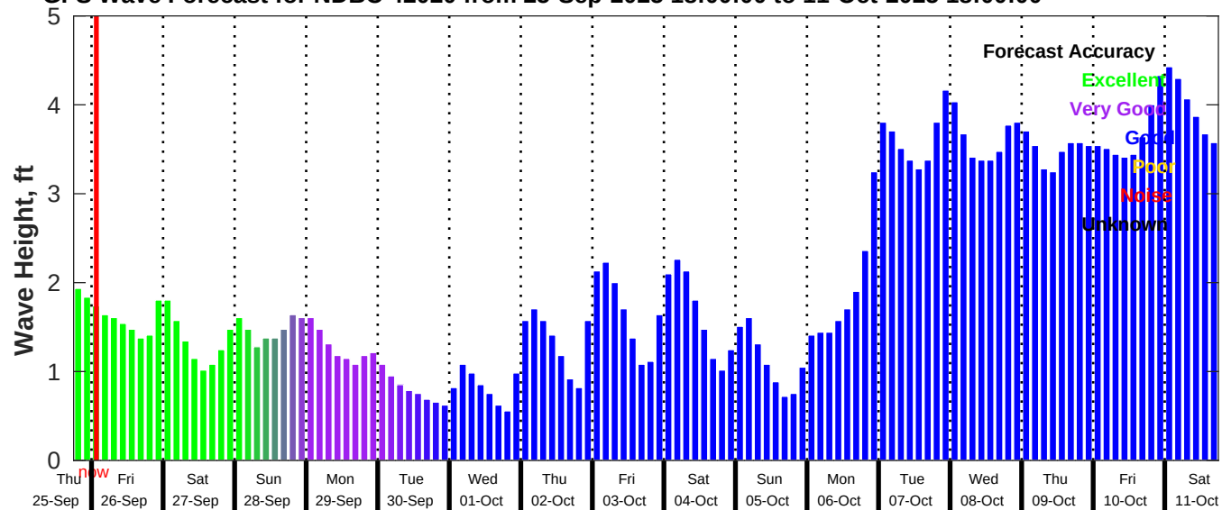
GFS Wave Forecast for NDBC 42020 from 25-Sep-2025 18:00:00 to 11-Oct-2025 18:00:00
