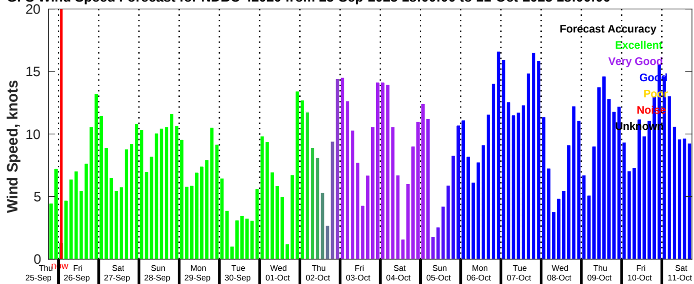
GFS Wind Speed Forecast for NDBC 42020 from 25-Sep-2025 18:00:00 to 11-Oct-2025 18:00:00
