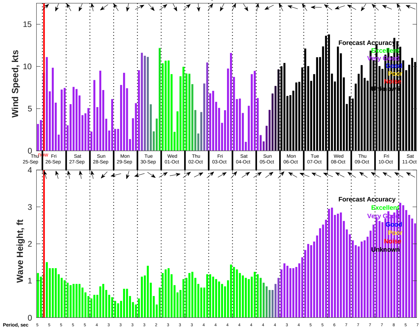
Wind & Wave Forecast for NDBC 42035 from 25-Sep-2025 18:00:00 to 11-Oct-2025 18:00:00
