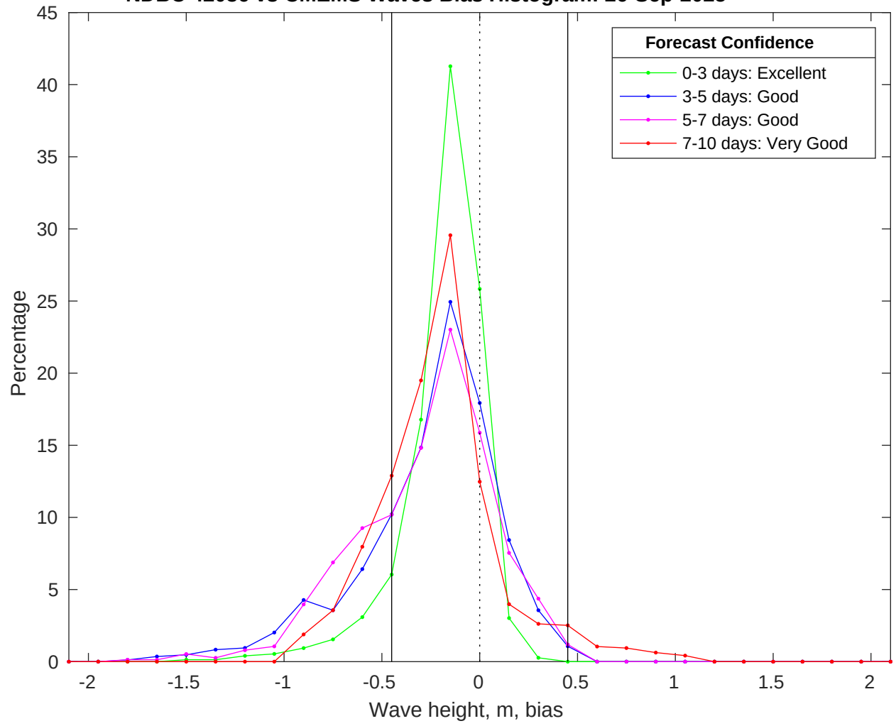
NDBC 42036 vs CMEMS Waves Bias Histogram: 26-Sep-2025
