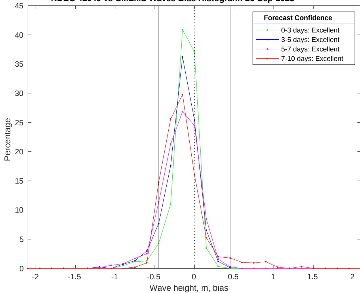
NDBC 42040 vs CMEMS Waves Bias Histogram: 26-Sep-2025
