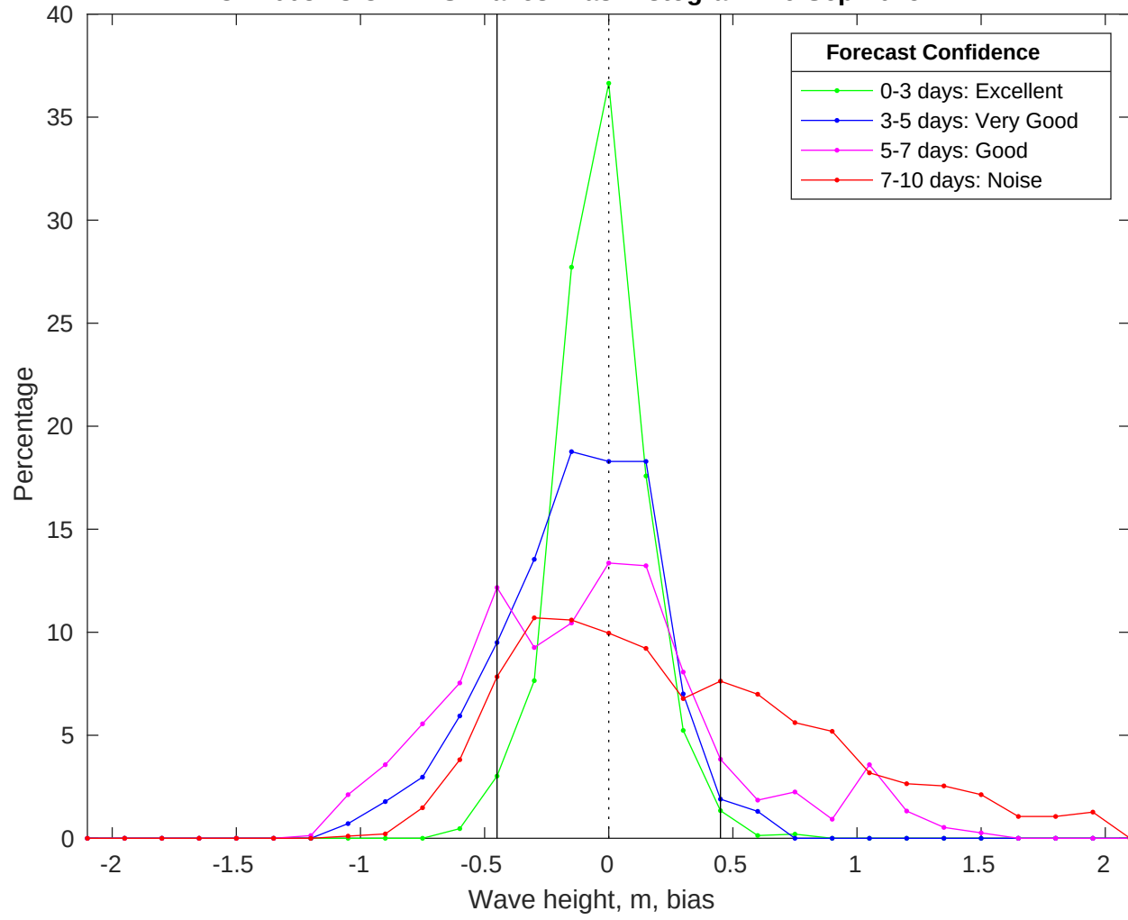
NDBC 44008 vs CMEMS Waves Bias Histogram: 26-Sep-2025
