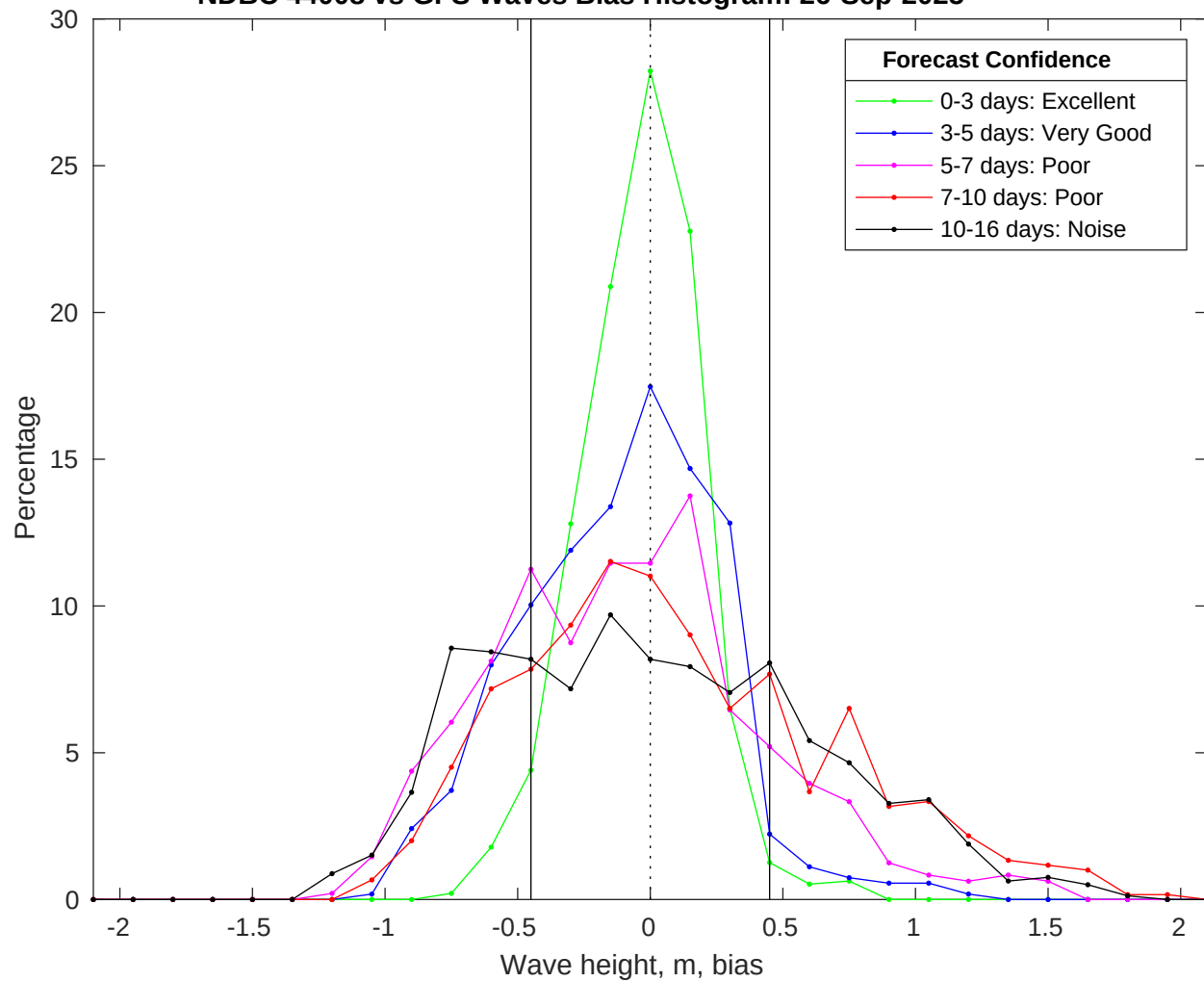
NDBC 44008 vs GFS Waves Bias Histogram: 26-Sep-2025
