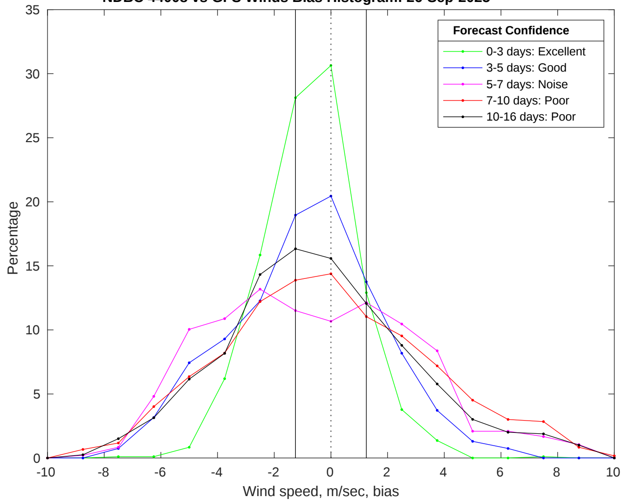
NDBC 44008 vs GFS Winds Bias Histogram: 26-Sep-2025
