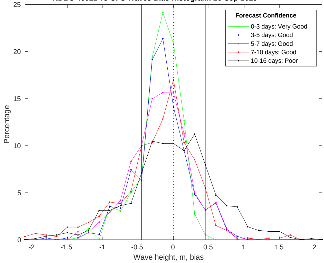
NDBC 46011 vs GFS Waves Bias Histogram: 26-Sep-2025
