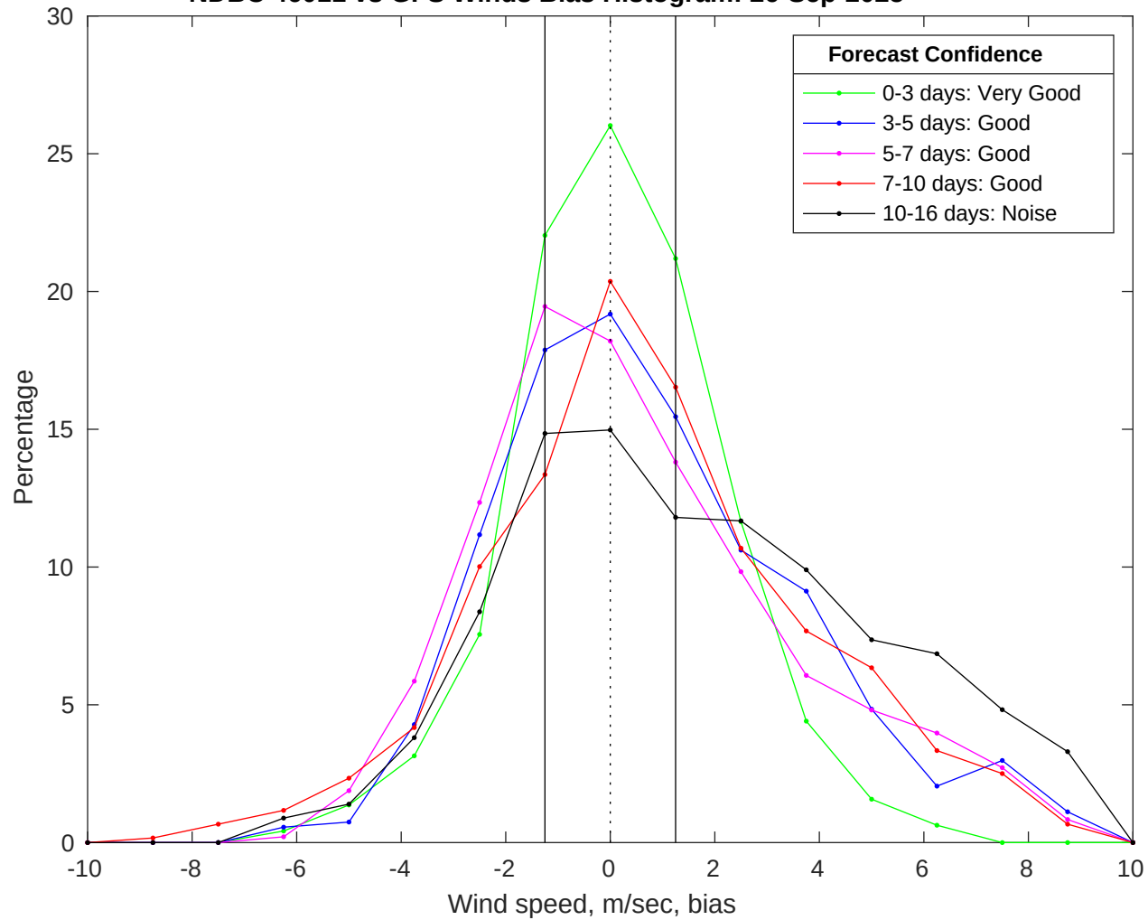
NDBC 46011 vs GFS Winds Bias Histogram: 26-Sep-2025
