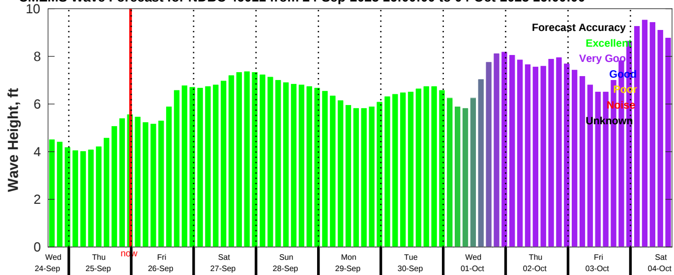
CMEMS Wave Forecast for NDBC 46011 from 24-Sep-2025 16:00:00 to 04-Oct-2025 16:00:00
