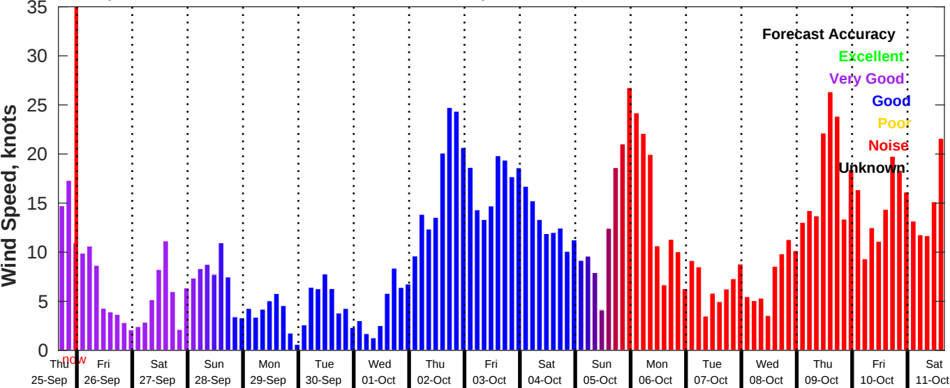
GFS Wind Speed Forecast for NDBC 46011 from 25-Sep-2025 16:00:00 to 11-Oct-2025 16:00:00
