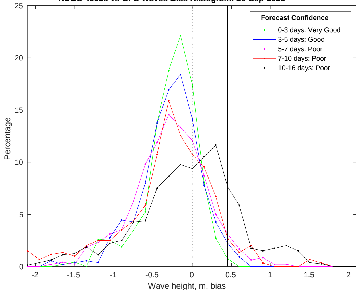
NDBC 46028 vs GFS Waves Bias Histogram: 26-Sep-2025
