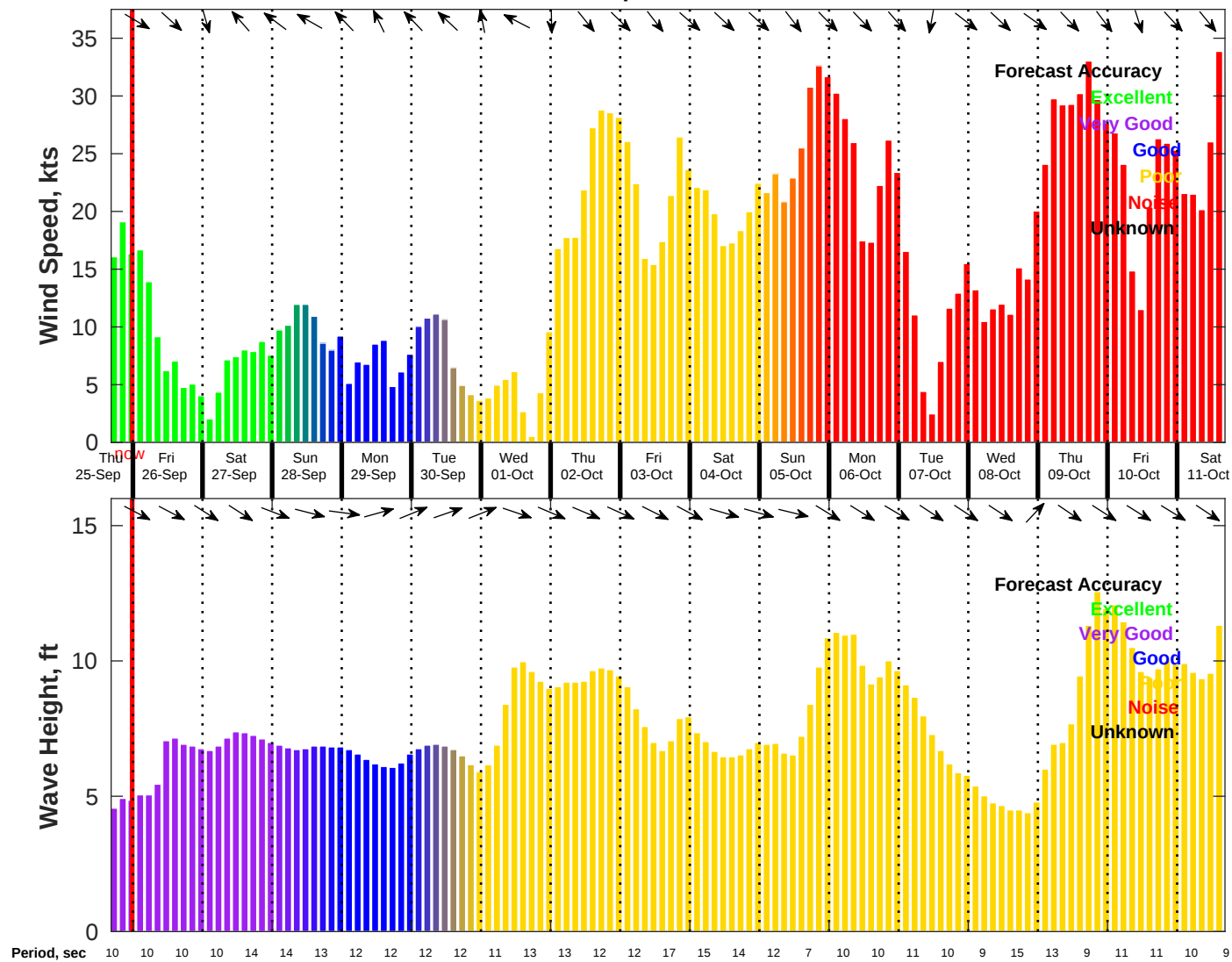
Wind & Wave Forecast for NDBC 46028 from 25-Sep-2025 16:00:00 to 11-Oct-2025 16:00:00
