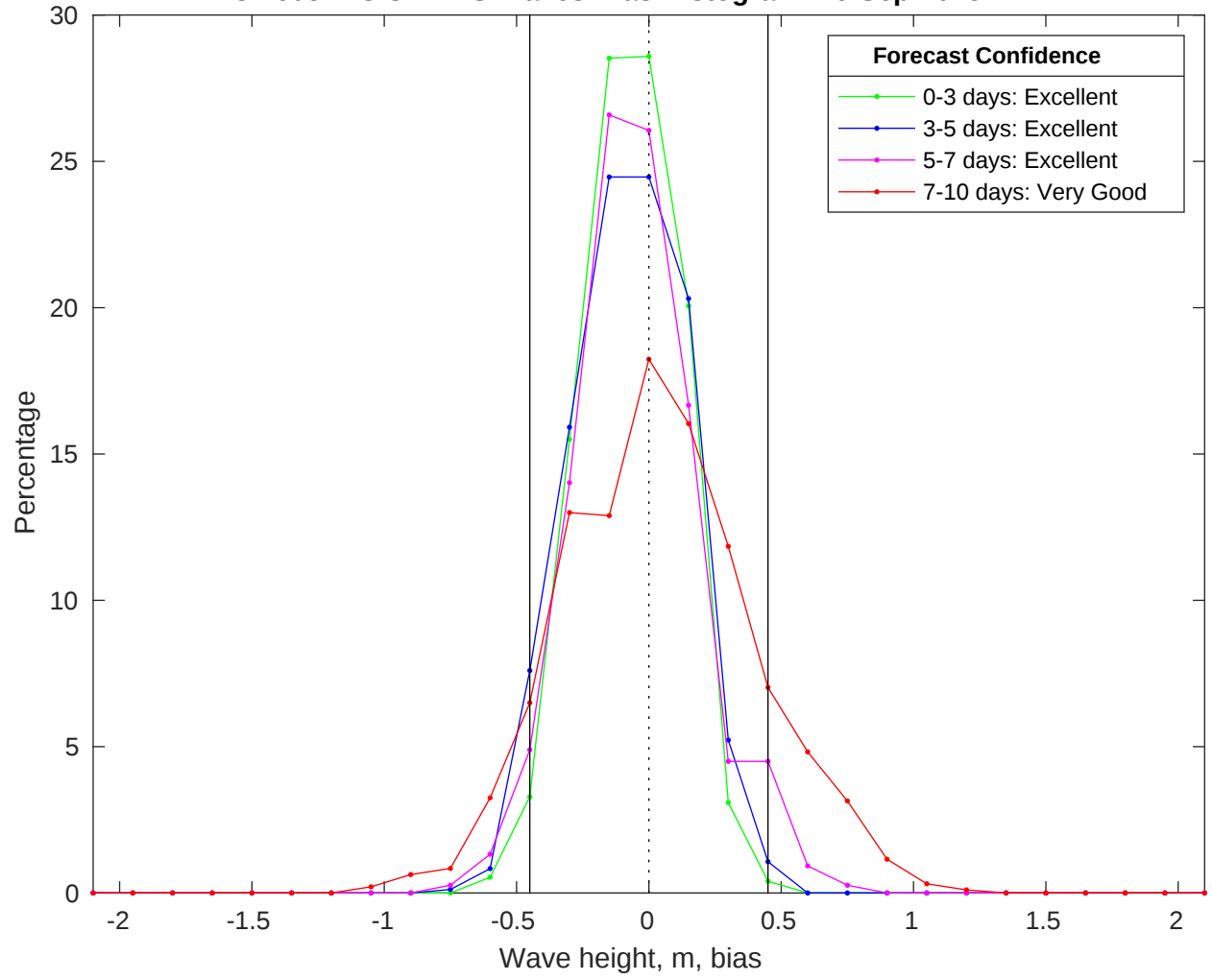
NDBC 46054 vs CMEMS Waves Bias Histogram: 26-Sep-2025
