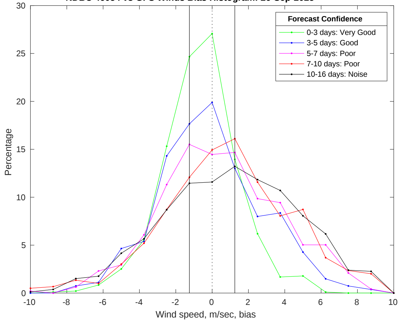
NDBC 46054 vs GFS Winds Bias Histogram: 26-Sep-2025
