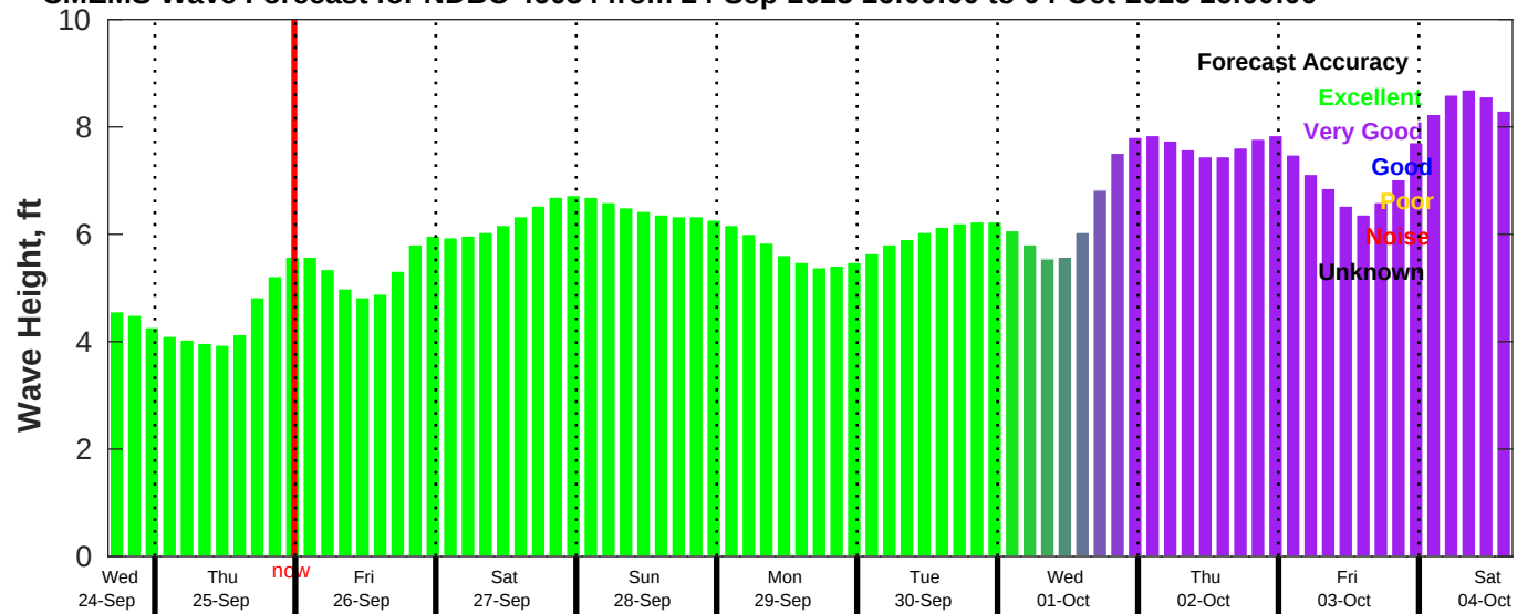
CMEMS Wave Forecast for NDBC 46054 from 24-Sep-2025 16:00:00 to 04-Oct-2025 16:00:00
