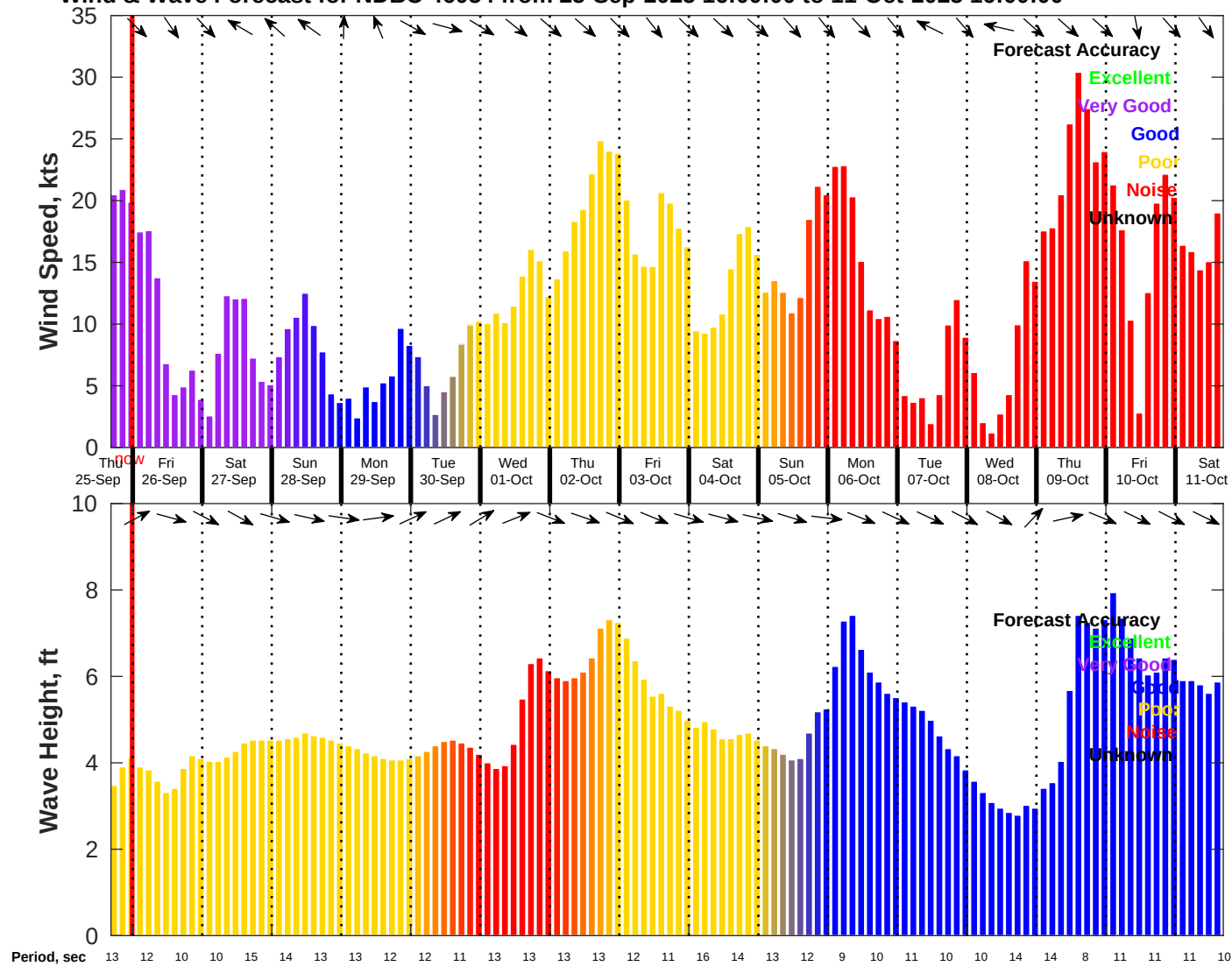
Wind & Wave Forecast for NDBC 46054 from 25-Sep-2025 16:00:00 to 11-Oct-2025 16:00:00
