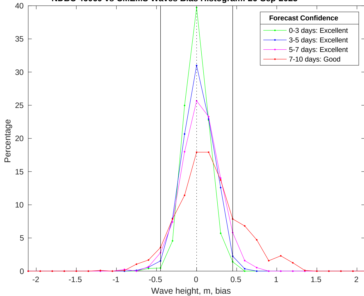
NDBC 46069 vs CMEMS Waves Bias Histogram: 26-Sep-2025
