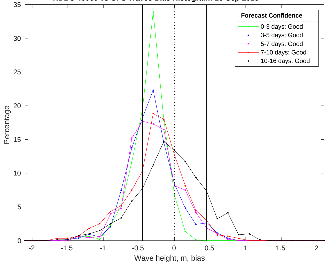
NDBC 46069 vs GFS Waves Bias Histogram: 26-Sep-2025
