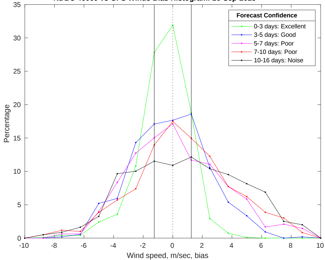
NDBC 46069 vs GFS Winds Bias Histogram: 26-Sep-2025
